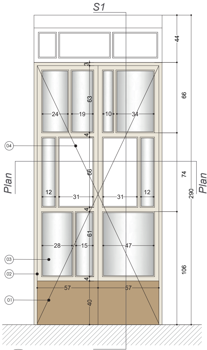
E.1 Front view S1 R-CA03 1:20
