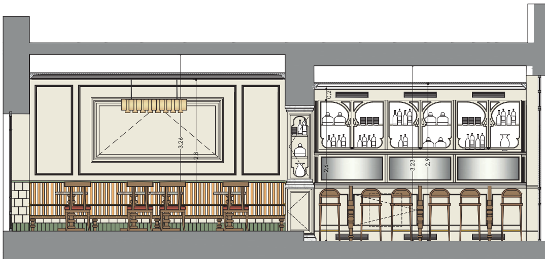
E.AA' Elevation AA'
