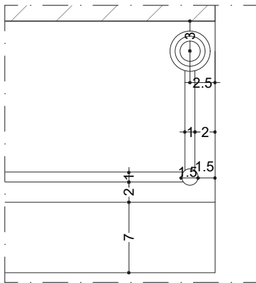
D3 Detail ML 5.03 1:5
