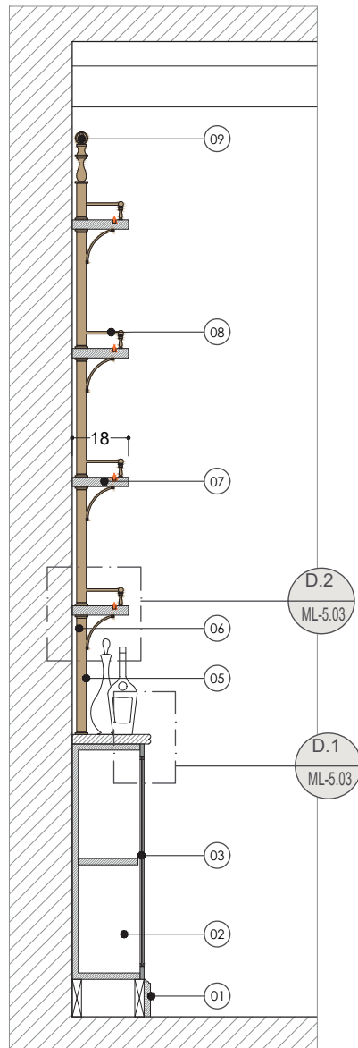
S Section ML 5.03
